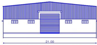
FRONT ELEVATION
