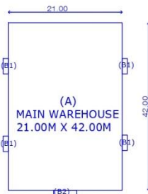
BLOCK PLAN
