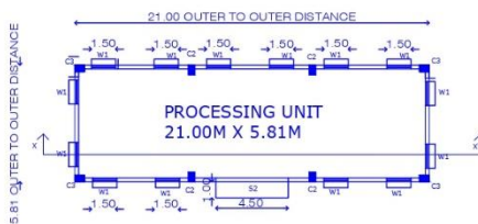
PLAN FOR PROCESSING UNIT
