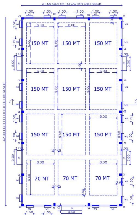
PLAN FOR 1560 MT.WH.
